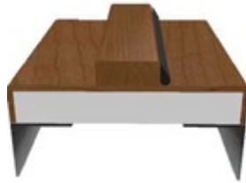
45 MINUTE: Veneered Fire Core (Shown with Optional Installation Angle Brackets)
