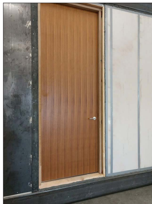
Sound Testing Grandoor Frames at Intertek Laboratories
